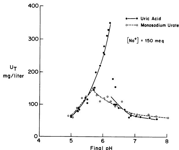
FIGURE 2 The comparison of HU solubility with that of NaU in 150 mM Na solution. After incubation of 5 mg of HU or monosodium urate monohydrate in each milliliter of solution (150 mM Na) used for 7 days, the U_T in ambient solution was determined.
