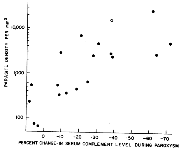
FIGURE 6 Correlation of parasite density with change in serum C' level during 18 paroxysms in relapse and one paroxysm of a primary attack ( r=0.76 ). The latter was one of only two primary paroxysms studied with CF antibody present.
