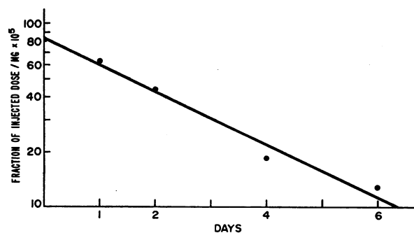
FIGURE 5 The specific activity time course of total biliary cholic acid after the intravenous injection of [ ^{24}\text{-}^{14}\text{C} ]Na glycocholate in subject E. Y. The line is the regression line obtained from a least squares fit of the data points.
