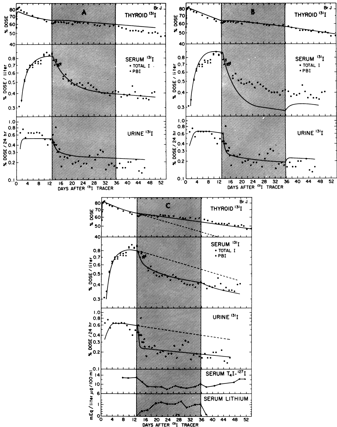
FIGURE 3 Comparison of computer solutions assuming different lithium effects, for patient Br. J. \text{Na-}^{131}\text{I} was given intravenously at time zero; the shaded area is the period of lithium administration. Solid circles and triangles represent measured data in 3A, 3B, and 3C. Solid lines (the \text{PB-}^{131}\text{I} line is omitted) are computer-generated least squares solutions generated under the following assumptions: 3A, lithium affected only iodine release; 3B, lithium affected only iodine release and no weight in the computer solution is to be given to serum data (that is, the curve is fitted only to thyroid and urine data); 3C, lithium affected both iodine release and hormone disappearance. The broken lines in 3C are the description of the behavior of the curves if lithium had not been given.
