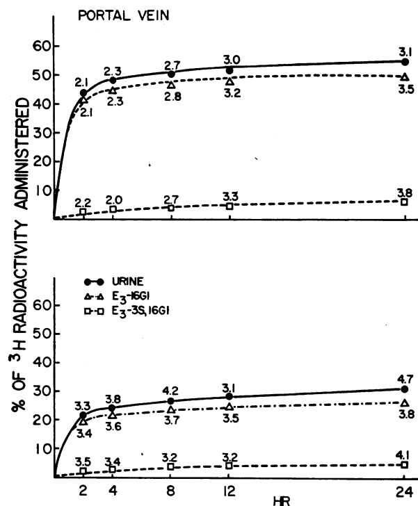
FIGURE 3 The cumulative urinary excretion of radioactive estriol conjugates after injection of ^3\text{H} -E 3 -16G1- ^{14}\text{C} ( ^3\text{H}/^{14}\text{C} ) of 2.1 (top) and 3.4 (bottom) into the portal vein system.
