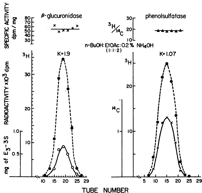
FIGURE 6 Characterization of ^3H-E_3-3S-16G1-^{14}C by partial enzymatic hydrolysis. Left: CCD of ^3H-E_3-3S formed by \beta -glucuronidase hydrolysis and of carrier E_3-3S . Right: CCD of ^3H-E_3-16G1-^{14}C formed by phenolsulphatase hydrolysis. In both cases 29 transfers were performed in system C (see Table II).
