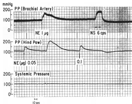
FIGURE 5 Changes in forelimb perfusion pressure (PP) and hind paw PP in response to intrabrachial NE and to nerve stimulation. The pressor response to NE in the forelimb was followed 20 sec later by a pressor response in the hind paw. There was no vasoconstriction in the hind paw during or after NS; instead a vasodilator response was seen in 50% of the experiments. The nature of this humoral dilator factor is not known. The amount of NE released from the paw during NS must be too small to be detected by this assay.
