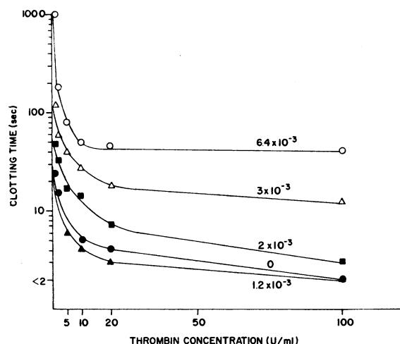
FIG. 1. EFFECT OF \alpha -TOCOPHEROL ON THE CLOT TIME OF CITRATED NORMAL PLATELET-RICH PLASMA AFTER ADDITION OF THROMBIN. To 0.3 ml of plasma, 0.1 ml of a solution of \alpha -tocopherol in 5% glucose was added, and the mixture was clotted with 0.1 ml of thrombin solution at 37° C. Final concentration of \alpha -tocopherol (M) is indicated on each line of the graph.
