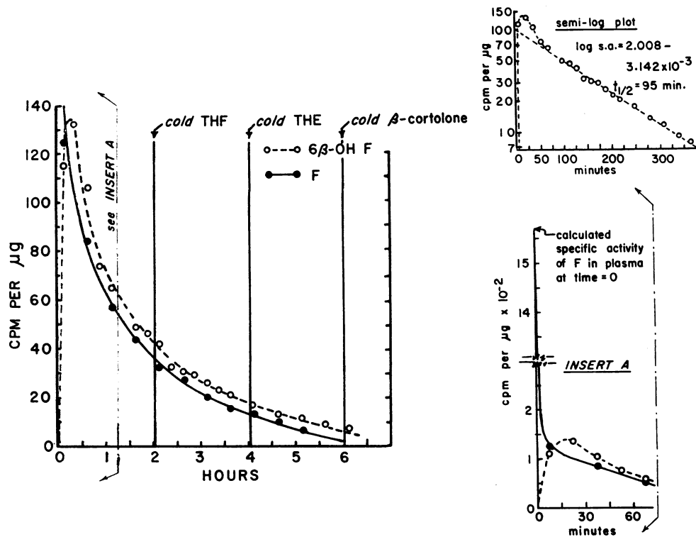
FIG. 9. SPECIFIC ACTIVITY OF 6 \beta -HYDROXYCORTISOL AS A FUNCTION OF TIME FOR THE CONTROL PERIOD. Insert A suggests a product-precursor relationship. Specific activity of F in plasma at time zero is total radioactivity administered/calculated plasma F content. Integral specific activity was determined from the area beneath the semi-log plot (see Figure 3), and from this the cortisol turnover was 177 mg per 24 hours. Turnover rate for 6 \beta -hydroxycortisol K = 0.693/t_{1/2} = 10.5 per 24 hours. Turnover is 10.5 N mg per 24 hours, where N (not determined) is pool size of 6 \beta -hydroxycortisol. Note maintenance of specific activities of cortisol and 6 \beta -hydroxycortisol after administration of unlabeled metabolites. 6 \beta -hydroxycortisol determined by acid phenylhydrazine reaction.
