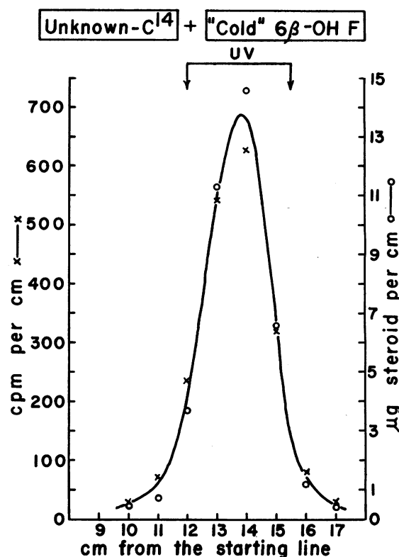
FIG. 8. PAPER CHROMATOGRAPHY OF A MIXTURE OF URINARY 6\beta -HYDROXYCORTISOL-4- C^{14} AND AUTHENTIC UNLABELED 6\beta -HYDROXYCORTISOL. Chromatographed in 90 per cent butanol in benzene: 50 per cent aqueous methanol overnight at 32^\circ\text{C} . Each centimeter strip was eluted for radioactivity and acid phenylhydrazine analyses.
