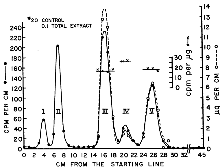
FIG. 4. PAPER CHROMATOGRAPHIC SEPARATION OF METABOLITES FROM ONE 15-MINUTE SAMPLE OF URINE. Each centimeter of paper eluted for analysis. Peaks III, IV, and V estimated by the acid phenylhydrazine reaction and identified further in Figure 5. I, cortols; II, cortolones; III, THF; IV, allo-THF; V, THE. 1 Sample is that analyzed in Table II. Chromatography was in the toluene-methanol system.
