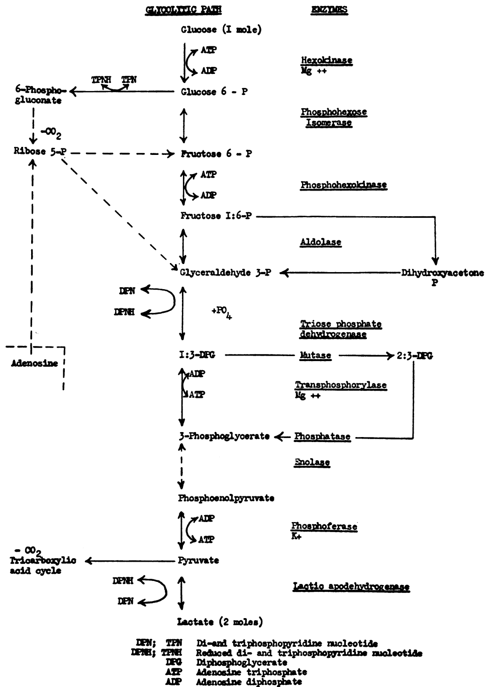
FIG. 1. DEGRADATION OF GLUCOSE TO LACTATE IN THE RED CELL
