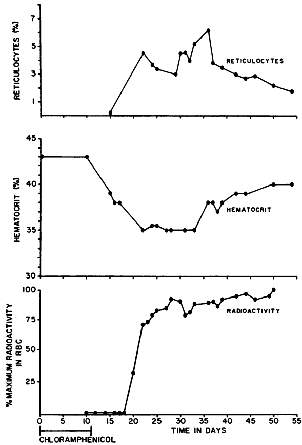
FIG. 2. EFFECT OF CHLORAMPHENICOL ON HEMATOCRIT, RETICULOCYTES AND APPEARANCE OF Fe 60 IN RED CELLS
