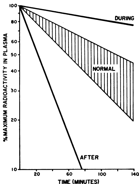
FIG. 1. THE EFFECT OF CHLORAMPHENICOL TOXICITY ON PLASMA DISAPPEARANCE OF Fe^{59}
