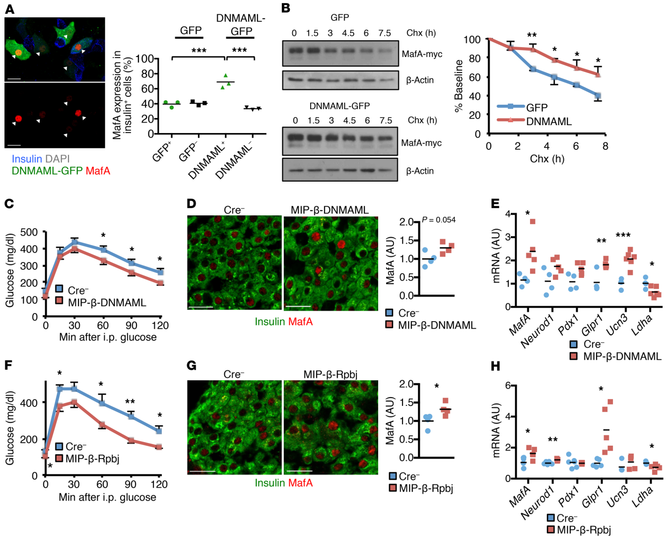
Figure 7. Notch loss of function stabilizes \beta cell MafA and improves glucose tolerance. (A) Representative image of islet cells dispersed from WT mice transduced with lentivirus expressing DNMAML-GFP (or GFP control) and exposed to 100 nM palmitate and 25 mM glucose for 72 hours. Arrows indicate DNMAML + cells. Quantitation shows insulin + MafA + islet cells in transduced vs. nontransduced cells ( n = 3 independent experiments). *** P < 0.001 , 1-way ANOVA and Dunnett's multiple comparisons post hoc test. (B) Western blots and quantification of residual MafA-Myc signal expressed as percentage of baseline from MIN6 cells with stable integration of DNMAML-GFP (or GFP control) transiently transfected with MafA-myc, then treated with 10 \mu\text{g/ml} cycloheximide (Chx) for the indicated times ( n = 3 independent experiments). * P < 0.05 ; ** P < 0.01 , 2-tailed t test. (C) GTT in TAM-treated, HFD-fed MIP- \beta -DNMAML and Cre - control mice ( n = 9 –11 mice/group) per experimental protocol shown in Supplemental Figure 8C. * P < 0.05 , 2-tailed t test. (D) Representative images and quantitation of MafA fluorescence intensity in pancreatic sections from HFD-fed MIP- \beta -DNMAML and Cre - control mice ( n = 4 mice/group). P = 0.054 , 2-tailed t test. (E) Gene expression in islets isolated from HFD-fed MIP- \beta -DNMAML and Cre - control mice ( n = 4 –5 mice/group). * P < 0.05 ; ** P < 0.01 ; *** P < 0.001 , 2-tailed t test. (F) GTT in HFD-fed MIP- \beta -Rbpj and Cre - control mice ( n = 9 mice/group). * P < 0.05 ; ** P < 0.01 , 2-tailed t test. (G) Representative images and quantitation of MafA fluorescence intensity in pancreatic sections from HFD-fed MIP- \beta -Rbpj and Cre - control mice ( n = 4 mice/group). * P < 0.05 , 2-tailed t test. (H) Gene expression in islets isolated from HFD-fed MIP- \beta -Rbpj and Cre - control mice ( n = 5 –6 mice/group). * P < 0.05 ; ** P < 0.01 , 2-tailed t test. Scale bars: 20 \mu\text{m} . All data are shown with group means \pm SEM.
