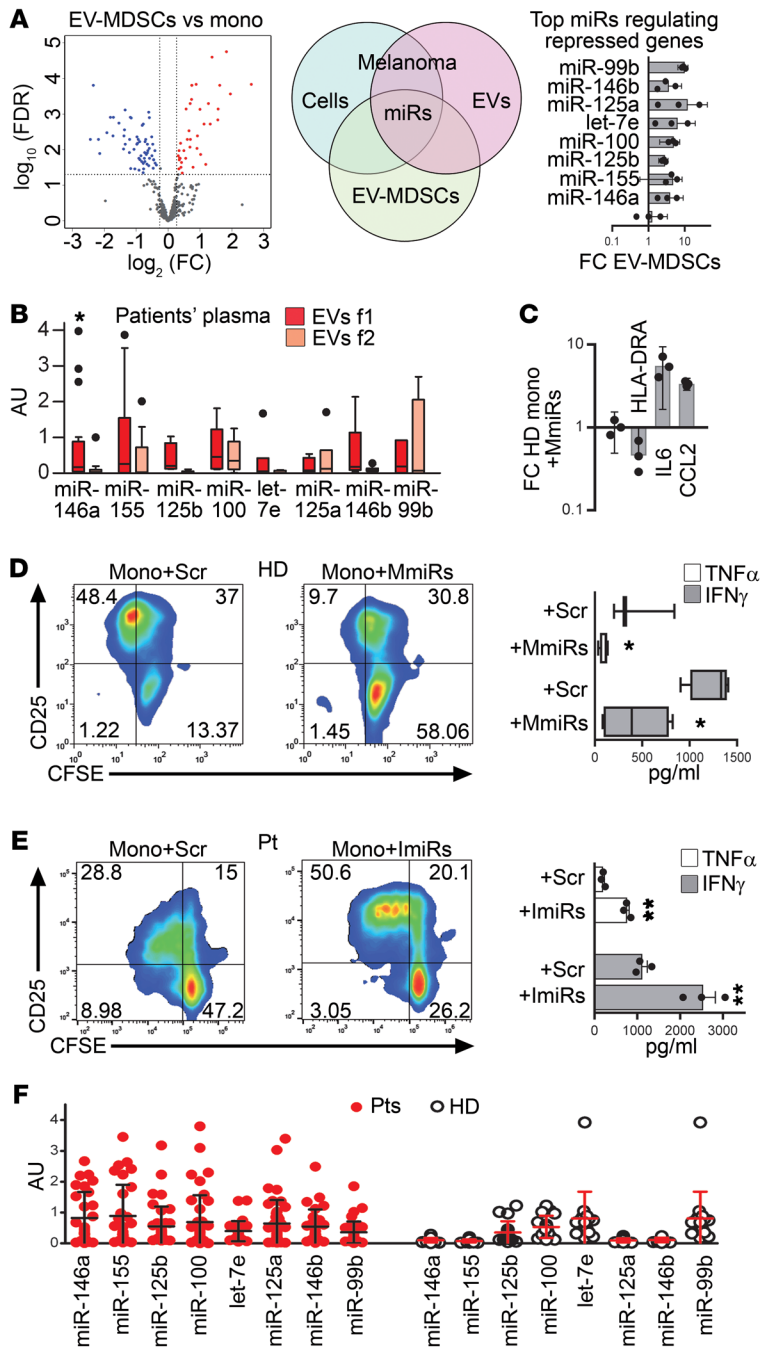
Figure 3. miR regulation in EV-MDSCs. (A) Volcano plot of the miRNAs regulated in EV-MDSCs ( n = 5 HD) compared with untreated monocytes based on microarray results, identification strategy of MDSC-miRs, and relative expression of selected miRNAs in EV-MDSCs compared with untreated monocytes assessed by qPCR in a representative HD. (B) Expression of MDSC-miRs in f1 and f2 plasma EVs of melanoma patients ( n = 16 ). Box and whiskers (Tukey's test). (C) Monocytes from HD transfected with MDSC-miR mimics (MmiRs) modulate HLA-DRA , IL6 , and CCL2 gene expression compared with monocytes treated with scrambled control used as calibrator. (D) Immunosuppressive activity of mono+MmiRs on autologous activated CFSE-labeled T cells, as evaluated by CD25 expression and proliferation (percentage is indicated, left), and release of IFN- \gamma and TNF- \alpha (right). (E) Loss of immunosuppressive activity of monocytes from a melanoma patient transfected with miR inhibitors (ImiRs) prior to cocubation with autologous activated CFSE-labeled T cells, as evaluated by flow cytometry (left) and cytokine release (right). (F) Expression of MDSC-miRs in CD14 + cells isolated from PBMCs of melanoma patients ( n = 31 ) and HD ( n = 15 ). AU, arbitrary units. P < 0.05 , paired Student's t test (A, C) and Mann-Whitney U test (F). * P < 0.05 ; ** P < 0.01 , paired Student's t test (B, D, E). Results are representative of 5 (C), 4 (D), and 3 (E) experiments.
