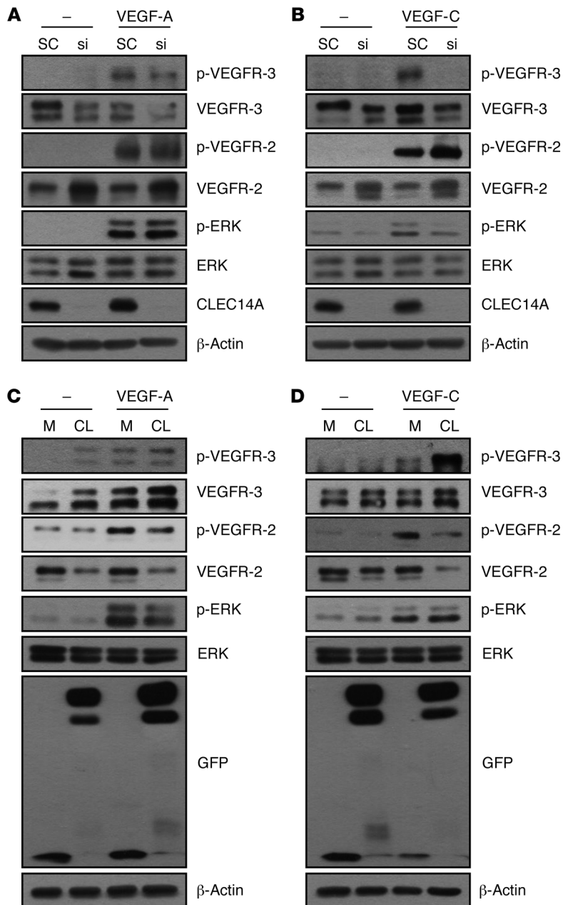
Figure 4. Silencing or overexpression of CLEC14A regulates the phosphoactivation of VEGFR-3 and VEGFR-2 and their downstream signaling upon stimulation with VEGF-C or VEGF-A in HDBECs. (A) Decreased phosphoactivation and expression of VEGFR-3 and increased phosphoactivation and expression of VEGFR-2 following increased phosphoactivation of ERK in HDBECs after knockdown of CLEC14A using siRNA (si) (50 nM) and treatment with 50 ng/ml VEGF-A for 5 minutes. (B) Decreased phosphoactivation and expression of VEGFR-3 following decreased phosphoactivation of ERK and increased phosphoactivation and expression of VEGFR-2 in HDBECs after knockdown of CLEC14A using siRNA (50 nM) and treatment with 100 ng/ml VEGF-C for 15 minutes. (C) Elevated phosphoactivation and expression of VEGFR-3 and reduced phosphoactivation and expression of VEGFR-2 following decreased phosphoactivation of ERK in HDBECs after overexpression of GFP-tagged CLEC14A, together with VEGF-A (50 ng/ml) for 5 minutes in HDBECs (GFP-Mock and GFP-CLEC14A-FL). (D) Enhanced phosphoactivation and expression of VEGFR-3 following increased phosphoactivation of ERK and decreased phosphoactivation and expression of VEGFR-2 after overexpression of GFP-tagged CLEC14A, together with VEGF-C (100 ng/ml) treatment for 15 minutes in HDBECs (GFP-Mock and GFP-CLEC14A-FL). All experiments were repeated in at least 4 different sets. M, mock transfected; CL, transfected with CLEC14A.
