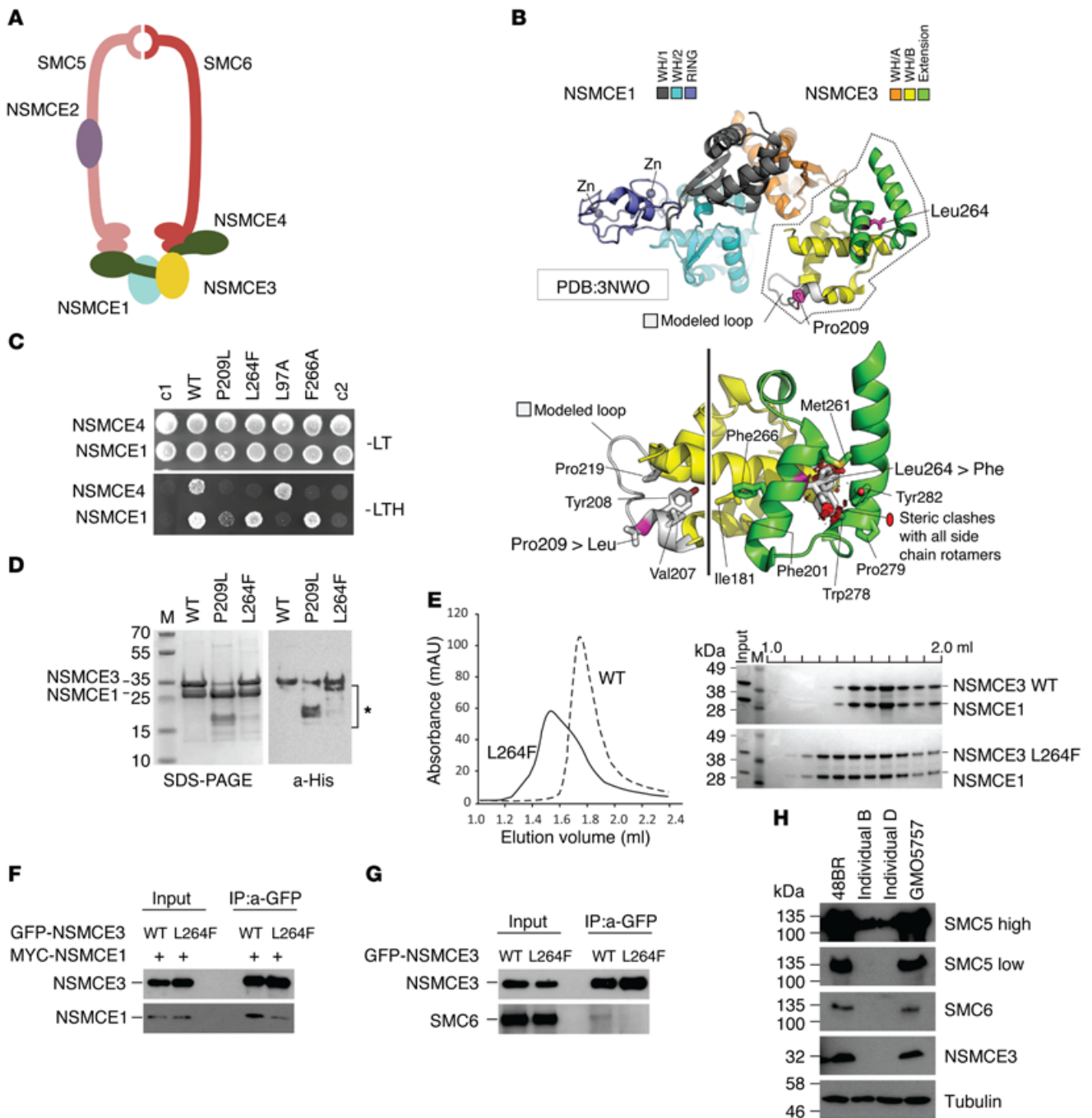
Figure 2. NSMCE3 mutations destabilize the SMC5/6 complex. (A) Schematic of the SMC5/6 complex. (B) Structure of NSMCE1/NSMCE3, highlighting the positions of the Leu264Phe (L264F) and Pro209Leu (P209L) mutants that destabilize the WH/B subdomain of NSMCE3. Loops missing from the deposited structure were modelled and are shown in gray (24). (C) Yeast 2-hybrid analysis showing interactions between NSMCE3 and NSMCE1 or NSMCE4, scored on His - plates containing 5 mM 3-amino-1,2,4-triazol (-LTH). WT denotes WT NSMCE3; L97A: NSMCE3 Leu97Ala, which abrogates NSMCE1 binding (25); F266A: NSMCE3 Phe266Ala, which reduces binding to NSMCE4 (21). L264F only interacts with NSMCE1; P209L has reduced interaction with NSMCE1 and no interaction with NSMCE4. Controls: c1, BD-NSMCE3 with empty AD vector; c2, empty BD vector with AD-NSMCE4 (top) or NSMCE1 (bottom). (D) NSMCE1 and His-tagged NSMCE3 (WT, P209L, and L264F) were coexpressed in, and purified from, E. coli . Left: Coomassie-stained SDS-PAGE shows copurification of NSMCE1 and NSMCE3. Right: Immunodetection of His-tagged NSMCE3. P209L is unstable; L264F is more stable. (E) Size exclusion chromatography column. NSMCE1 and NSMCE3 co-elute, forming a stable complex. NSMCE1 and L264F co-elute, over a broader range of volume and non-uniform distribution, indicating either unfolding of L264F or interaction with the chromatography resin. (F) GFP-tagged NSMCE3 (WT or L264F) and Myc-tagged NSMCE1 were ectopically expressed in human U205 osteosarcoma cells; proteins were stable and full length in input samples. Proteins were immunopurified using anti-GFP beads. Purification of NSMCE1 was reduced when copurified with L264F, which indicated reduced affinity. (G) GFP-tagged NSMCE3 (WT or L264F) was ectopically expressed in U205 cells. Proteins were immunopurified using anti-GFP beads. Reduced copurification indicates a compromised integration of the mutated NSMCE3 into the SMC5/6 complex. (H) Western blot analysis of SMC5/6. NSMCE3 is undetectable in fibroblasts from individual B (GVH02) and individual D (FCP488) compared with primary fibroblast cell lines (48BR and GM05757). High exposure of anti-SMC5 blot shows reduction of SMC5. Levels of both SMC5 and SM6 were reduced in patient fibroblasts, indicating destabilization of the complex. Loading control: tubulin.
