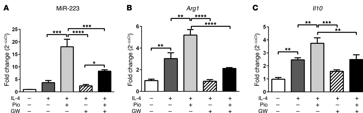
Figure 1. miR-223 expression is induced in PPAR \gamma -dependent M2 macrophage activation. Expression of miR-223 (A), arginase 1 ( Arg1 ) (B), and IL-10 ( Il10 ) (C) in WT BMDMs in the presence of IL-4 with or without pioglitazone (Pio) or PPAR \gamma antagonist GW9662 (GW) for 48 hours ( n = 3 ). Data are presented as the mean \pm SEM. ** P < 0.01 , *** P < 0.001 , and **** P < 0.0001 by 1-way ANOVA with Bonferroni's post test.
