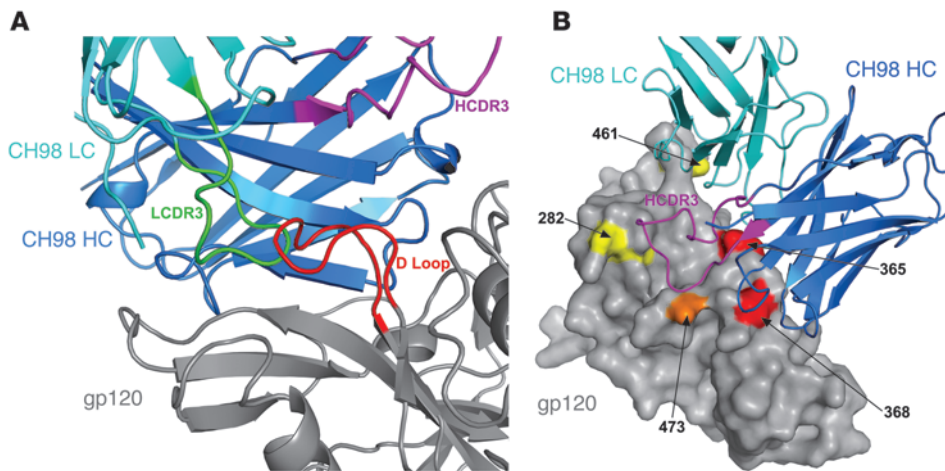
Figure 3 Threading of CH98 onto the gp120 complexed structures of CD4bs VRC01 and CH103 BnAbs. (A) CH98 model based on threading onto the gp120 complexed VRC01 crystal structure. The CH98 heavy chain (HC; dark blue) and light chain (LC; light blue) threaded onto the VRC01 structure complexed with gp120 (gray) resulted in an incompatible model, with a clash between the gp120 D loop (red) and the LCDR3 (green). (B) CH98 model based on threading onto the gp120 complexed CH103 crystal structure. The CH98 heavy chain (dark blue) and light chain (light blue) threaded onto the CH103 structure complexed with gp120 (gray) resulted in a model in which HCDR3 (magenta) dominates the binding to the CD4bs region and engages in direct contact with gp120 residues in positions 365, 368, 473, and 282, all of which affect CH98 binding. The residue in position 461 makes direct contact with LCDR1. Each residue that affects CH98 binding in the epitope mapping is illustrated using the corresponding color in Figure 2.
