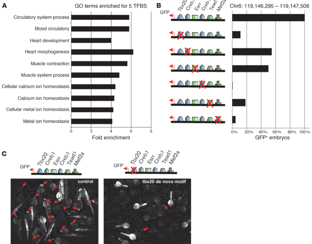
Figure 6 Cooccurrence of transcription factor-binding motifs for Tbx20 , Mef2a , Tead1 , Esrr , and Creb1 is important for gene expression regulation of ion transport genes. (A) Top10 enriched GO terms for peaks containing the combination of 5 TFBS. (B) Independent mutagenesis of motifs located in Tbx20 peaks near Cacna1c gene. (C) Mutagenesis of Tbx20 de novo motif shows abrogation of enhancer function (right) compared with control (left). Arrows point to Cacna1c enhancer driving expression of the reporter gene GFP in transgenic zebrafish heart.
