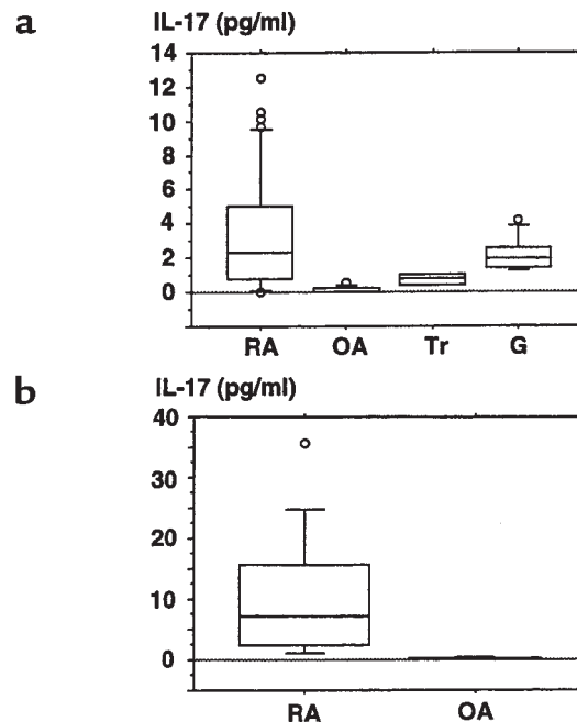
Figure 8 Concentrations of IL-17 in the synovial fluids (a) or culture media of synovial tissues (b) from RA, OA, trauma, and gout patients. Synovial fluids were obtained from 43 RA, 9 OA, 4 trauma, and 7 gout patients (a). Synovial tissues were obtained from 12 RA and 3 OA patients (b). A part of the tissue was dissected into small pieces (1 g), rinsed well with PBS (pH 7.4), and cultured in 1 mL of RPMI-1640 containing 100 U/mL of penicillin, 10 \mu g/mL of streptomycin, and 2 mM L-glutamine for 3 days in 5% CO 2 in air at 37°C. Culture media were collected, and their concentrations of IL-17 were measured using a ELISA kit for human IL-17. The mean value of the concentration of IL-17 of 3 synovial pieces from a single joint was calculated. The results are expressed as box plots, as described in Methods. Significant differences between RA and OA: P < 0.0001 (a); P < 0.009 (b). Tr, trauma; G, gout.
