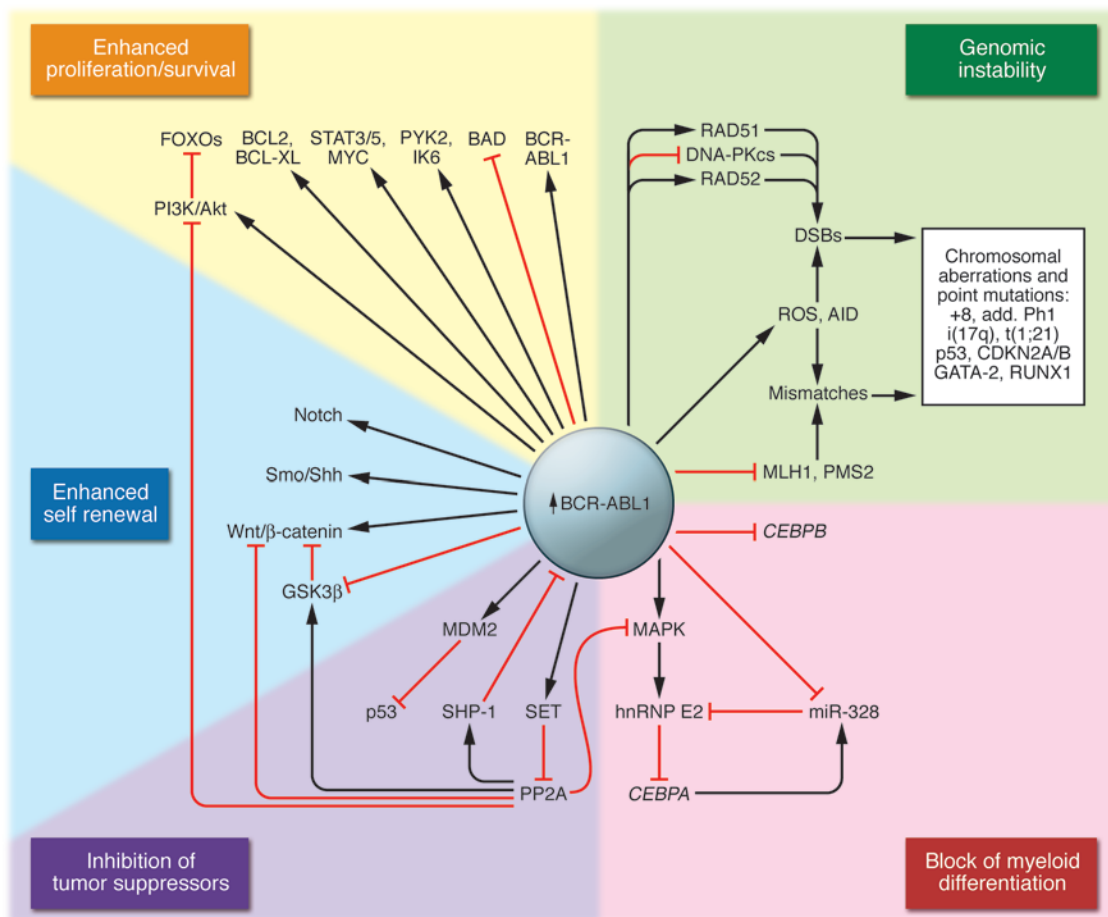
Figure 1 BCR-ABL1–dependent pathways to blastic transformation. Schematic representation of the potential BCR-ABL1–dependent molecular mechanisms leading to CML disease progression. The relatively high BCR-ABL1 expression/activity in CML-CP CD34 + CD38 - stem cells and/or CD34 + early progenitors compared with more committed progenitors, which is further markedly increased in CML-BP CD34 + progenitors results in the following: enhancement of proliferation/survival pathways; increased genomic instability; and activation of pathways leading to a block in myeloid differentiation, acquisition of the ability to self renew, and inhibition of tumor suppressors with broad cell regulatory functions. BAD, BCL2 antagonist of cell death; DNA-PKcs, DNA-dependent protein kinase, catalytic subunit; FOXO, forkhead box O; IK6, Ikaros 6; miR-328, microRNA-328; MLH1, mutL homolog 1; PMS2, postmeiotic segregation increased 2; RAD51, RecA homolog in Escherichia coli ; RAD52, RAD52 homolog ( Saccharomyces cerevisiae ); Shh, Sonic Hedgehog; wnt/β-catenin, wingless-int1/beta-catenin.
