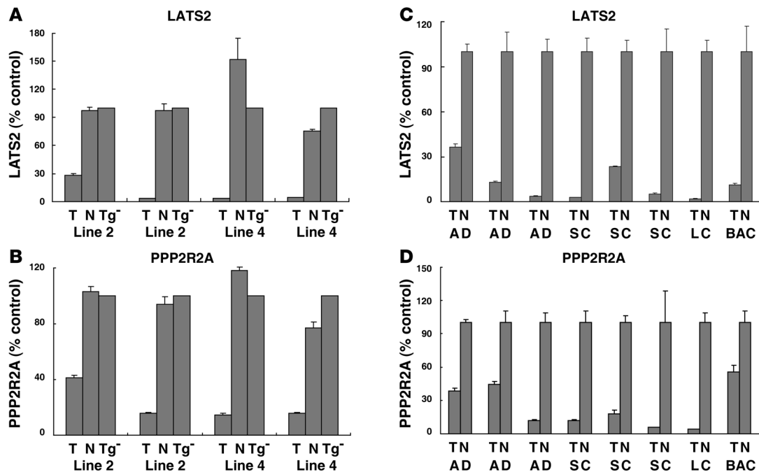
Figure 8 Validation of LATS2 and PPP2R2A expression profiles by real-time RT-PCR assays performed on RNA isolated from the indicated murine cyclin E-transgenic lines and from the paired human normal-malignant lung tissues. Real-time RT-PCR assays for (A) LATS2 and (B) PPP2R2A were performed. Results were normalized to expression within nontransgenic FVB mouse lung tissues. Real-time RT-PCR assays for (C) LATS2 and (D) PPP2R2A were independently performed on paired human normal-malignant lung tissues. Results were normalized to expression in normal human lung tissues. In all groups, P values were less than 0.001. Error bars indicate SD.
