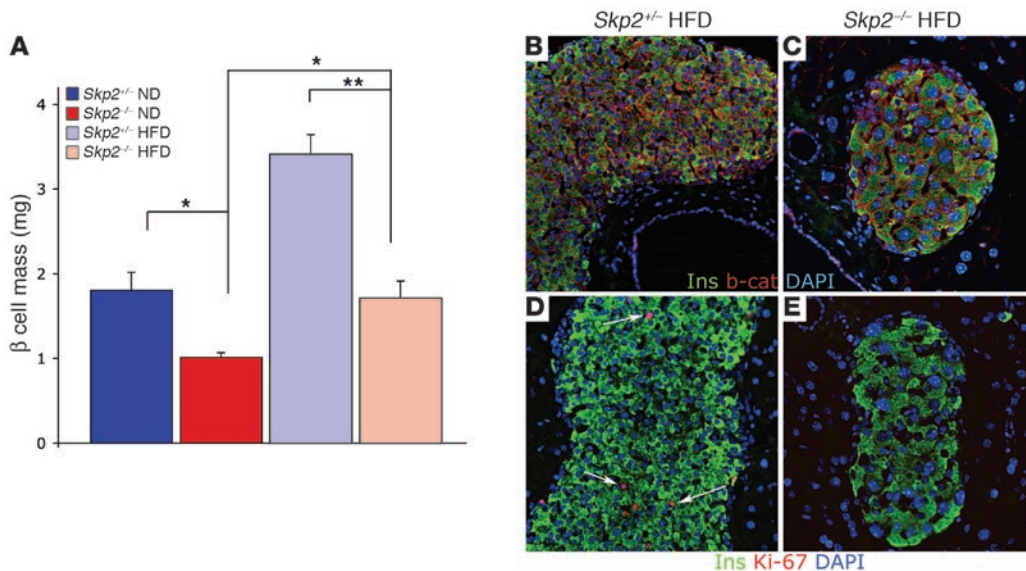
Figure 7 Adaptive expansion of \beta cell mass was abrogated in Skp2^{-/-} mice. (A) Analysis of \beta cell mass 12 weeks after feeding with HFD or ND. n = 3 per group. (B–E) Pancreatic sections from Skp2^{+/-} mice (B and D) and Skp2^{-/-} mice (C and E) fed HFD for 12 weeks were immunostained with antibodies to insulin (green) and to \beta -catenin (red) (B and C), or to insulin (green) and Ki-67 (red) (D and E). Arrows denote proliferating \beta cells. DAPI-stained nuclei appear blue. * P < 0.05 ; ** P < 0.01 .
