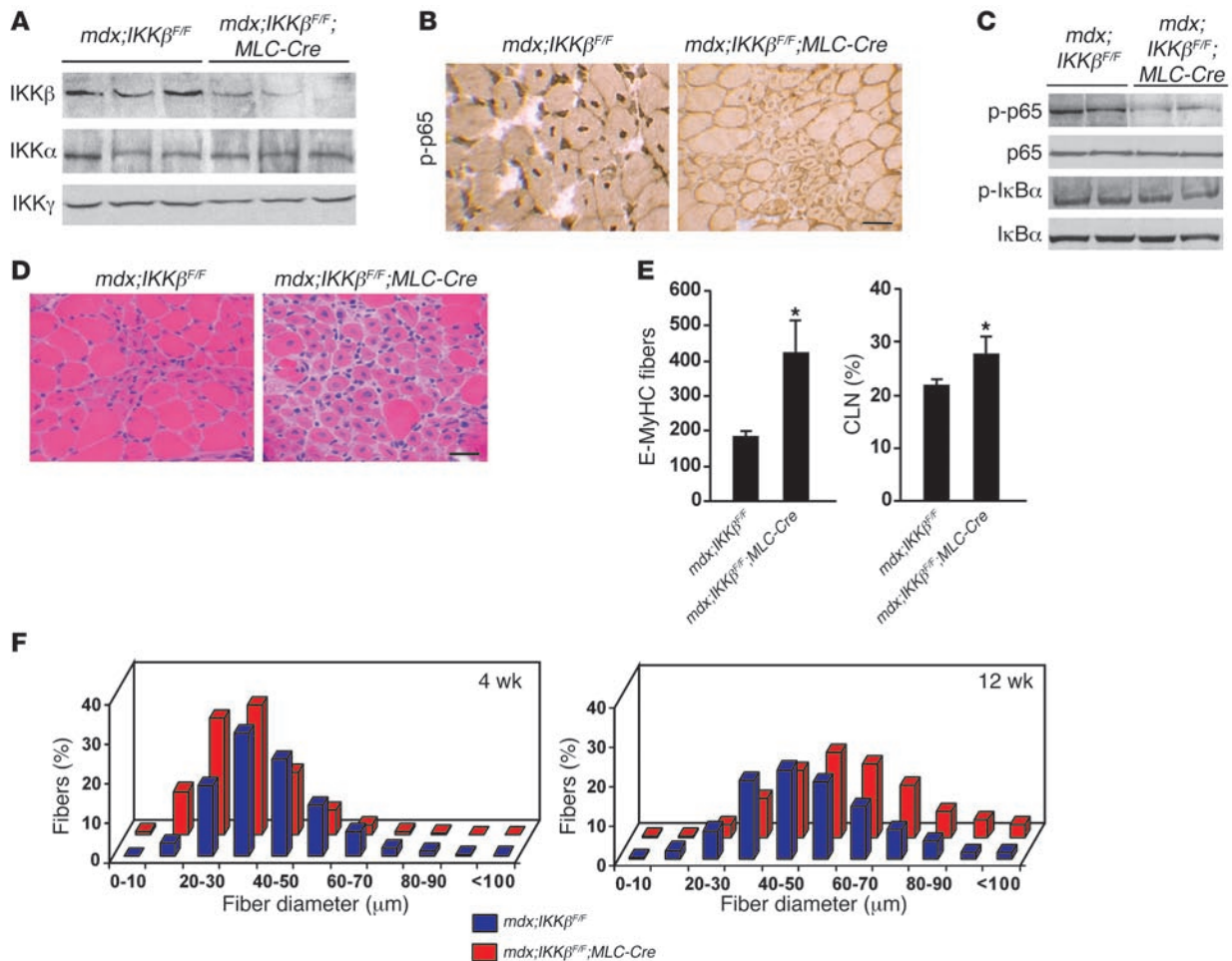
Figure 6 IKK \beta deletion in muscle cells promotes regeneration. Muscles harvested from 4-week- (A–F) or 12-week-old (F only) mdx;IKK \beta^{F/F} and mdx;IKK \beta^{F/F};MLC-Cre mice were used for protein analysis (A and C) or histology (B and D). (A) Western blots probing for IKK subunits. (B) Muscles were immunostained for p-p65 expression. (C) Western blots probing for p-p65, p65, and I \kappa B \alpha . (D) H&E staining of mdx;IKK \beta^{F/F} and mdx;IKK \beta^{F/F};MLC-Cre muscles. (E) Muscles used in D were stained for quantitation of E-MyHC–positive stained fibers or stained with H&E for counting of CLN. * P < 0.05 . Scale bars: 15 \mu m (B) and 50 \mu m (D). Graphs are plotted as mean \pm SEM. (F) Mean fiber distribution in mdx;IKK \beta^{F/F} and mdx;IKK \beta^{F/F};MLC-Cre mice was determined from a minimum of 3,000 fibers from randomly chosen fields, obtained from multiple muscle sections from a minimum of 4 mice per group.
