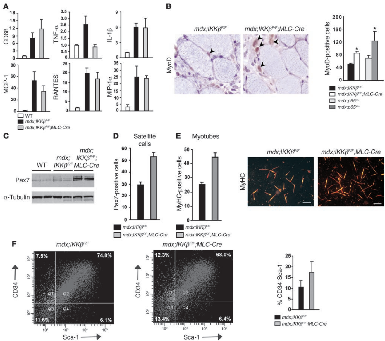
Figure 7 Muscle progenitor cells increase in mice lacking IKK \beta . Gastrocnemius or quadriceps were harvested from 4-week-old mdx;IKK \beta^{F/F} and mdx;IKK \beta^{F/F};MLC-Cre mice and frozen for RNA analysis (A), cryosectioned (B), or homogenized for immunoblotting (C). (A) Real-time PCR analysis of CD68, TNF- \alpha , IL-1 \beta , MCP-1, RANTES, and MIP-1 \alpha (macrophage inflammatory protein 1 \alpha ) obtained from 3–6 mice per group. (B) Sections as described in A or from 7-week-old mdx;p65 +/+ and mdx;p65 +/- mice were immunostained with MyoD and quantitated from a minimum of 20 randomly chosen fields per section in 3–4 animals per group. (C) Western blots probing for Pax7 and \alpha -tubulin. (D and E) Satellite cells were isolated from pooled hind limb muscles from 4-week-old mdx;IKK \beta^{F/F} and mdx;IKK \beta^{F/F};MLC-Cre littermates and either fixed and stained with Pax7 or differentiated for 3 days and subsequently stained with MyHC to determine myotube number normalized per mm 2 area. Scale bars: 200 \mu m. (F) Flow-cytometric analysis from freshly isolated cells of 4-week-old mdx;IKK \beta^{F/F} and mdx;IKK \beta^{F/F};MLC-Cre mice were stained with cell-surface markers CD34 and Sca-1. Graph represents averages from 2 independent experiments. Data are plotted as mean \pm SEM.
