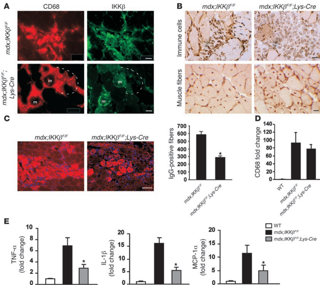
Figure 5 IKKβ deletion in myeloid cells reduces inflammation. (A and B) Gastrocnemius sections from 4-week-old mdx;IKKβ FF and mdx;IKKβ FF ;Lys-Cre male mice were analyzed either by double immunofluorescence staining against IKKβ (green) and CD68 (red) (A) or by immunohistochemistry for p-p65 (B). Dashed white lines in A mark field of macrophages. m, muscle fibers. Scale bars: 10 μm. (B) p-p65 immunohistochemical staining of immune infiltrates (top row) and regenerating muscle fibers (bottom row). Scale bars: 15 μm (top) and 10 μm (bottom). (C) Necrotic fibers were identified by IgG staining (filled fibers in red, nuclei in blue) (n = 6). Scale bar: 50 μm. Quantification of necrosis appears in the graph. (D) Real-time PCR analysis of CD68 in TA from sex- and age-matched WT, mdx;IKKβ FF and mdx;IKKβ FF ;Lys-Cre mice. (E) Real-time PCR analysis was performed as described in D for TNF-α, IL-1β, and MCP-1. Graphs are plotted as mean ± SEM. *P < 0.05.
