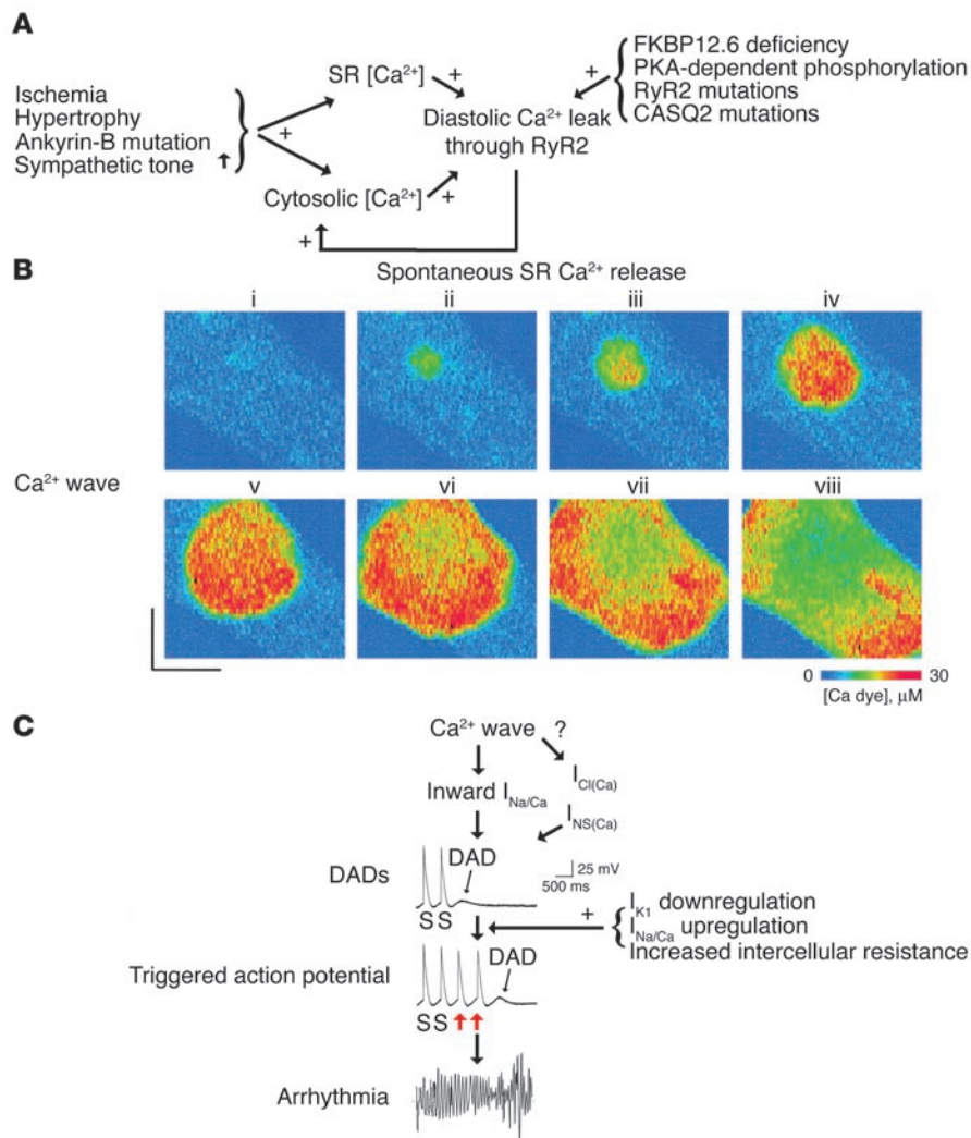
Figure 3 Proposed scheme of events leading to DADs and triggered tachyarrhythmia. (A) Congenital (e.g., ankyrin-B mutation) and/or acquired factors (e.g., ischemia, hypertrophy, increased sympathetic tone) will cause a diastolic \text{Ca}^{2+} leak through RyR2, resulting in localized and transient increases in [\text{Ca}^{2+}]_i in cardiomyocytes. (B) Representative series of images showing changes in [\text{Ca}^{2+}]_i during a \text{Ca}^{2+} wave in a single cardiomyocyte loaded with a \text{Ca}^{2+} -sensitive fluorescent dye. Images were obtained at 117-ms intervals. Focally elevated \text{Ca}^{2+} (ii) diffuses to adjacent junctional SR, where it initiates more \text{Ca}^{2+} release events, resulting in a propagating \text{Ca}^{2+} wave (iii–viii). Reproduced with permission from Biophysical Journal (85). (C) The \text{Ca}^{2+} wave, through activation of \text{Ca}^{2+} -sensitive inward currents, will depolarize the cardiomyocyte (DAD). In cardiomyocytes, the inward I_{\text{Na}/\text{Ca}} is the major candidate for the transient inward current underlying DADs, although the role of the \text{Ca}^{2+} -activated \text{Cl}^- current [ I_{\text{Cl}(\text{Ca})} ] and a \text{Ca}^{2+} -sensitive nonspecific cation current [ I_{\text{NS}(\text{Ca})} ] cannot be excluded. If of sufficient magnitude, the DAD will depolarize the cardiomyocyte above threshold resulting in a single or repetitive premature heartbeat (red arrows), which can trigger an arrhythmia. Downregulation of the inward rectifier potassium current ( I_{\text{K}1} ), upregulation of I_{\text{Na}/\text{Ca}} , or a slight increase in intercellular electrical resistance can promote the generation of DAD-triggered action potentials. S, stimulus. Modified with permission from Circulation Research (26) and Nature (12).
