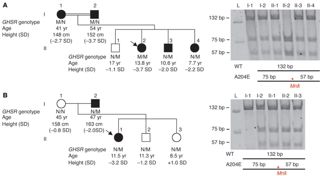
Figure 2 Inheritance of the A204E GHSR mutation in families 1 and 2. (A) Family 1. (B) Family 2. Circles and squares denote female and male family members, respectively. The SD to mean height for age is given below each symbol; height values are before GH treatment. Black symbols denote a short stature. The probands are indicated by arrows. The segregation of the GHSR A204E allele within both families was carried out by means of a specific restriction fragment length polymorphism (the A204E mutation creates an Mnl I site).
