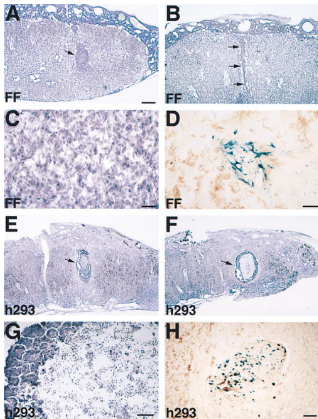
Figure 4. Bright-field microphotographs of frontal sections through primary fibroblast (A–D) or h293 cell (E–H) grafts. (A and B) Nissl staining illustrating the morphology of two different fibroblast grafts (arrows) at E21. In contrast to RE131 cell grafts, the limits of fibroblast grafts are easy to delineate. (C) High magnification of a Nissl-stained fibroblast graft at E21. (D) High magnification of a \beta gal-positive fibroblast graft at E21. (E and F) Nissl-staining illustrating the morphology of two different h293 cell grafts (arrows) at E17. (G) High magnification of the graft illustrated in (F) showing the large number of Nissl-stained inflammatory cells. (H) High magnification of a \beta gal-positive h293 cell graft 6 d after grafting in the placenta (E17). FF, Primary rat fibroblasts. Scale bar: 500 \mu m in A, B, E, and F; 45 \mu m in C; 50 \mu m in D; 41 \mu m in G; and 86 \mu m in H.
