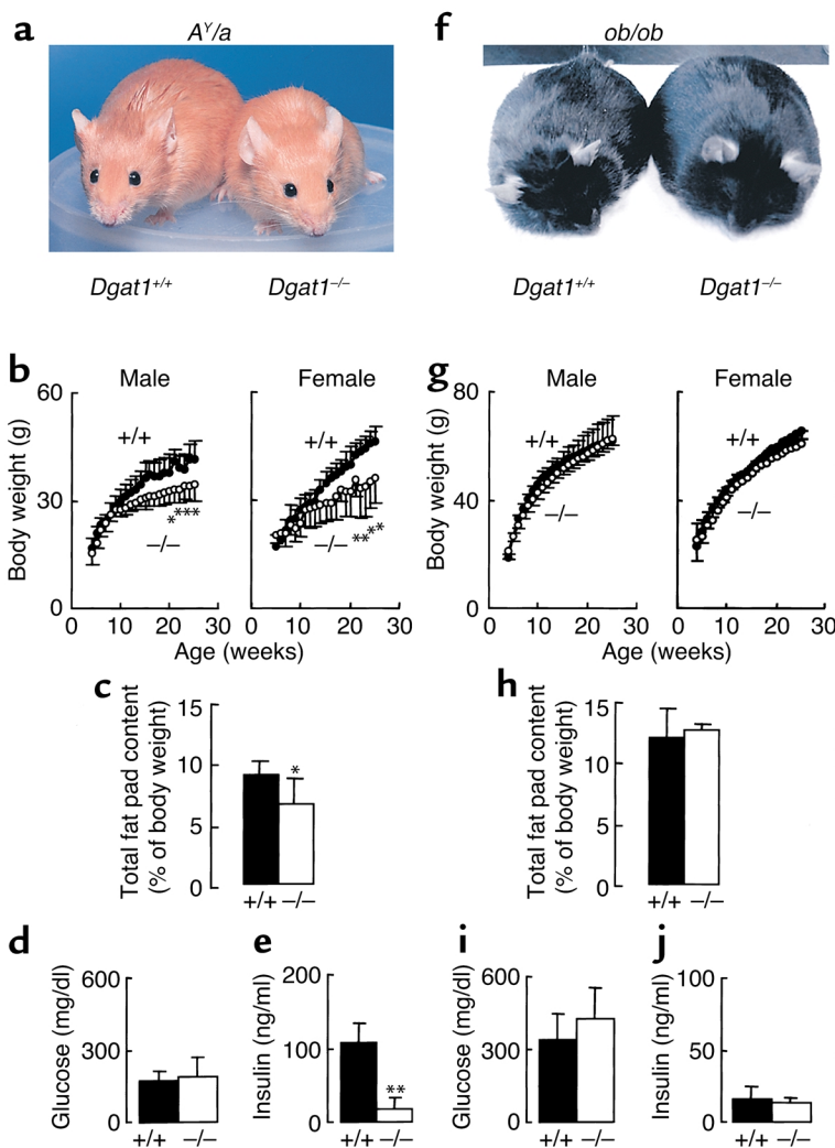
Figure 5 Effects of DGAT1 deficiency on energy and glucose metabolism in Agouti yellow ( A^Y/a ) and leptin-deficient ( ob/ob ) mice. n = 8-12 mice per genotype for growth curves, n = 5 chow-fed male mice per genotype for fat pad content, and n = 4-6 chow-fed male mice per genotype for plasma glucose and insulin concentrations. * P < 0.05 , ** P < 0.01 versus Dgat1^{+/+} mice.
