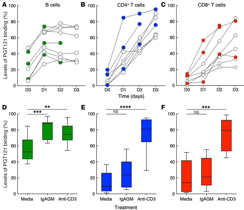
Figure 2. Time course of PGT121 binding to B cells and CD4+ and CD8+ T cells of HIV-infected and -uninfected individuals following cellular activation. Levels of PGT121 binding to B cells (A), CD4+ T cells (B), and CD8+ T cells (C) in PBMCs from HIV-infected (filled circles) and -uninfected (empty circles) individuals, at days 0, 1, 2, and 3 after stimulation with anti-CD3. Levels of PGT121 binding to B cells (D), CD4+ T cells (E), and CD8+ T cells (F) following 2-day stimulation of PBMCs of HIV-uninfected individuals using B cell-specific (IgAGM) and T cell-specific (anti-CD3) stimulation. Cells incubated without any stimulus (media) served as baseline. Statistical significance was tested with Friedman’s ANOVA. ** P < 0.01; *** P < 0.001; **** P < 0.0001. NS, not significant.
