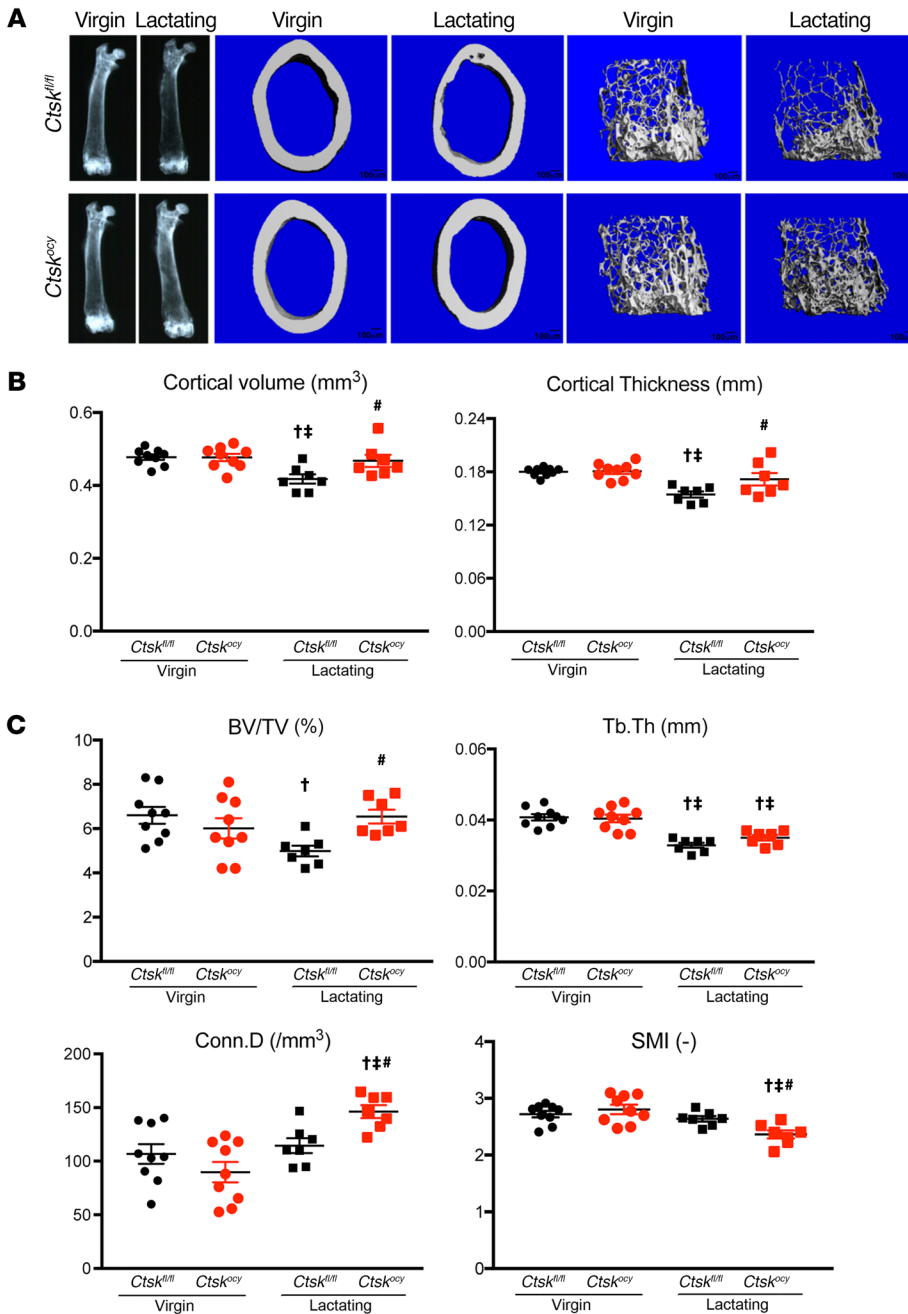
Figure 3. Deletion of Ctsk in osteocytes preserves cortical and cancellous bone during lactation. (A) Representative x-ray and \mu CT images of virgin and lactating Ctsk fl/fl and Ctsk ocv femurs ( n = 7-9 per group). Scale bars: 100 \mu m. (B) \mu CT analysis of cortical bone at the femoral midshaft of virgin and lactating Ctsk fl/fl mice (black dots and squares, respectively) and Ctsk ocv mice (red dots and squares, respectively) ( n = 7-9 per group). (C) \mu CT analysis of trabecular bone at the distal femur of virgin and lactating Ctsk fl/fl (black dots and squares, respectively) and Ctsk ocv (red dots and squares, respectively) mice ( n = 7-9 per group). Results represent the mean \pm SEM. † P < 0.05 versus virgin Ctsk fl/fl mice; ‡ P < 0.05 versus virgin Ctsk ocv mice; and # P < 0.05 versus lactating Ctsk fl/fl mice; 2-way ANOVA followed by Fisher's PLSD test.
