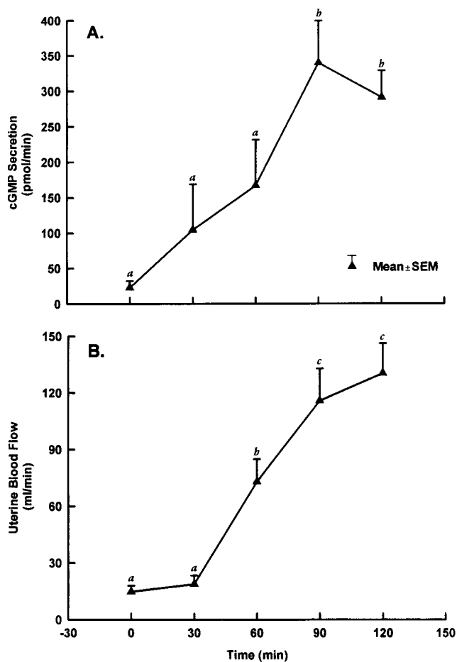
Figure 1. Pattern of change in uterine secretion of cGMP (A) and uterine blood flow (B) after the systemic intravenous infusion of 1 \mu\text{g}/\text{kg} E_2\beta ( n = 7 ) in nonpregnant sheep. Different letters denote differences between time periods at P < 0.001 by ANOVA.
