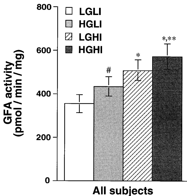
Figure 2. Glucose and insulin treatment of HSMC increases GFA activity. HSMC cultures were treated for 4 d during fusion and differentiation with 5 mM glucose and 22 pM insulin (low glucose-low insulin, LGLI), 20 mM glucose and 22 pM insulin (high glucose-low insulin, HGLI), 5 mM glucose and 30 \mu\text{M} insulin (LGHI), or 20 mM glucose and 30 \mu\text{M} insulin (HGHI), and their extracts were assayed for in vitro GFA activity. GFA activity from HSMC of all subjects is shown as mean \pm SEM under each treatment. # P < 0.05 , * P < 0.005 compared to LGLI, and ** P < 0.005 compared to HGLI by Student's paired t test.
