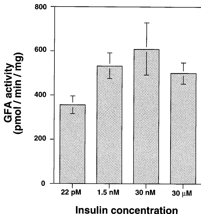
Figure 3. Insulin treatment of HSMC leads to a dose-dependent increase in GFA activity. HSMC were treated for 4 d during fusion and differentiation with 5 mM glucose and varying concentrations of insulin. Shown are the mean and SEM from HSMC from six subjects.
