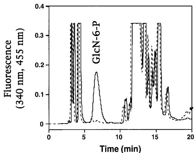
Figure 1. HPLC determination of glucosamine-6-phosphate. GFA activity was assayed in vitro (see Methods). GlcN-6-P generation was quantitated by fluorescent derivatization and HPLC separation. GlcN-6-P production was completely inhibited in the presence of 500 \mu\text{M} UDP-GlcNAc (dashed line).
