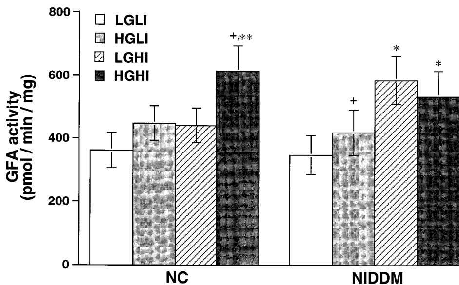
Figure 4. GFA activity and regulation by glucose and insulin is similar in HSMC from NC and NIDDM muscle. The data from Fig. 2 are divided into nondiabetic control (NC) and NIDDM cultures. HSMC GFA activities of all subjects is shown as means \pm SEM. +P < 0.025 , *P < 0.01 compared to LGLI, and **P < 0.005 compared to HGLI by Student's paired t test.
