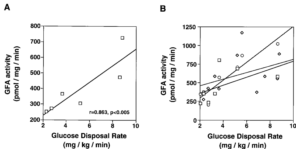
Figure 6. In contrast to NC, GFA activity is positively correlated with glucose disposal rate in NIDDM. (A) GFA activity assayed from NIDDM HSMC treated with low glucose and low insulin is shown. (B) GFA activities from NIDDM HSMC cultured in the other three glucose and insulin conditions are plotted against the subjects' GDR.
