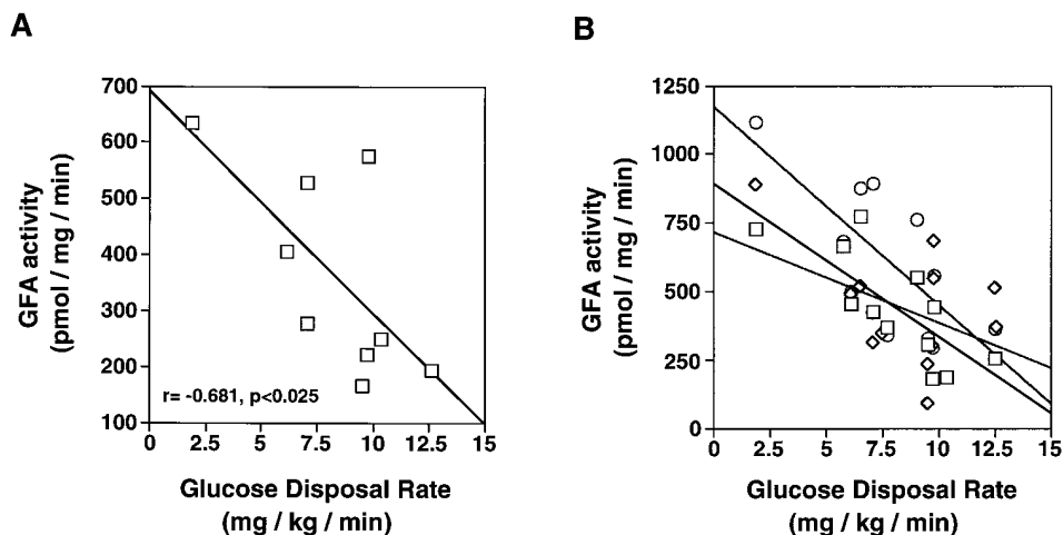
Figure 5. GFA activity is negatively correlated with glucose disposal rate in nondiabetic subjects. (A) GFA activity assayed from NC HSMC treated with low glucose and low insulin is shown as a function of the subject's GDR determined in vivo by means of a hyperinsulinemic euglycemic clamp. (B) GFA activities from HSMC cultured in the other three glucose and insulin conditions (see Fig. 2 legend) are plotted against the subject's GDR.
