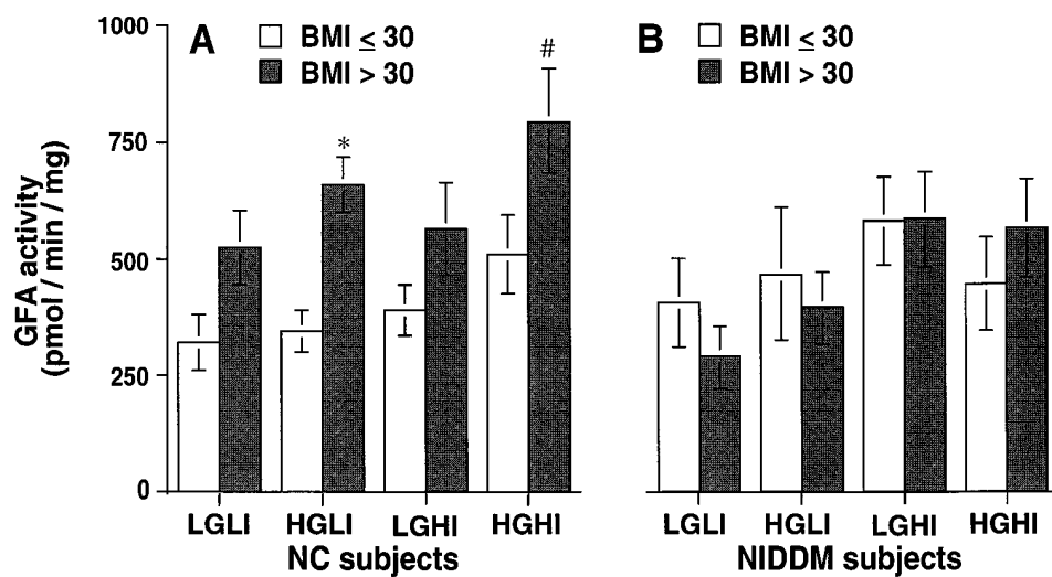
Figure 7. GFA activity as a function of body mass index. GFA activity was determined in HSMC from nondiabetic control (A) and NIDDM (B) subjects treated with the indicated concentrations of glucose and insulin for 4 d during fusion and differentiation. Mean GFA activity \pm SEM is shown for subjects with BMIs \leq 30 (open bars [NC: LGLI, n = 7 ; HGLI, n = 8 ; LGHI, n = 9 ; HGHI, n = 7 ; NIDDM: LGLI, n = 4 ; HGLI, n = 3 ; LGHI, n = 4 ; HGHI, n = 3 ]) compared to subjects with BMIs > 30 (filled bars [NC: LGLI, n = 2 ; HGLI, n = 4 ; LGHI, n = 4 ; HGHI, n = 4 ; NIDDM: LGLI, n = 4 ; HGLI, n = 6 ; LGHI, n = 8 ; HGHI, n = 7 ]). # P < 0.05 , * P < 0.005 compared to GFA activity in HSMC from subjects with BMIs \leq 30 treated with the same concentrations of glucose and insulin (Student's t test).
