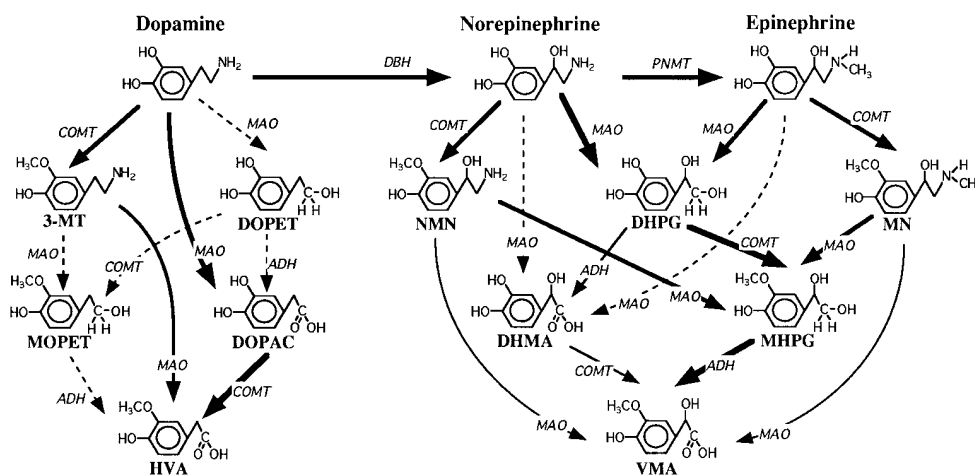
Figure 1. The metabolic pathways of degradation of NE, EPI, and DA. The deaminated metabolites are DHPG, DOPAC, dihydroxy-mandelic acid (DHMA), dihydroxy-phenylethanol (DOPET), methoxyhydroxyphenylethanol (MOPET), HVA, MHPG, and VMA. The O-methylated amine metabolites are normetanephrine (NMN), metanephrine (MN), and 3-MT. DBH, DA \beta -hydroxylase; PNMT, phenylethanolamine-N-methyltransferase; ADH, alcohol dehydrogenase.
