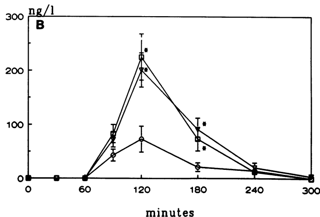
Figure 1. Serum levels of TNF (A) and IL-6 (B) after the intravenous administration of endotoxin (4 ng/kg). The results of the intravenous administration of endotoxin alone ( \square ) are compared with the results of the combined infusion of endotoxin (4 ng/kg) and pentoxifylline ( \circ ) or of the combined infusion of endotoxin (4 ng/kg) and 600 \mu\text{g/kg} anti-tissue factor monoclonal antibody ( \nabla ). Mean values and SD are given, statistical significance ( P < 0.05 ) as compared to the chimpanzees receiving endotoxin alone is indicated (*).
