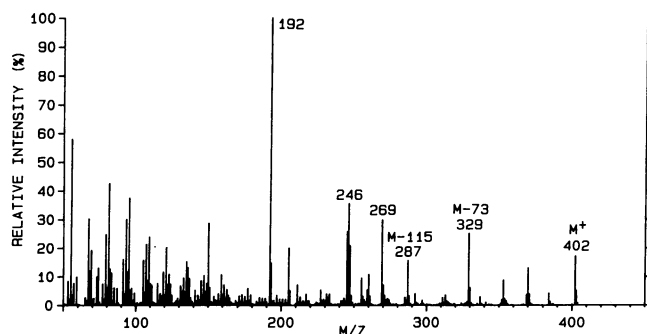
Figure 3. Electron impact mass spectrum of the methyl 3,7-dioxo-cholanoate obtained by chromic acid oxidation of alloisoursodeoxy-cholic acid liberated from urinary bile acid N -acetylglucosaminides.
