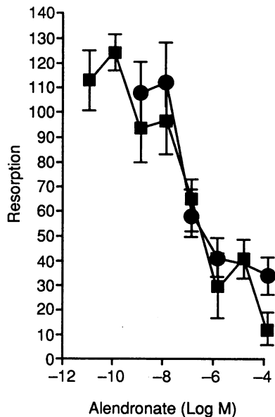
Figure 7. Alendronate effects on the resorption activity of isolated osteoclasts. The effect of alendronate on the resorption activity of chicken osteoclasts (●) was compared with the effects on rat osteoclastic activity (■); see Sato and Grasser (42). Chicken osteoclasts were isolated from hens as described by Zamboni-Zallone et al. (50), while rat osteoclasts were examined as described in Sato and Grasser (42). In both systems alendronate inhibited bone resorption with an IC_{50} = 0.1 \mu M . Chicken resorption
