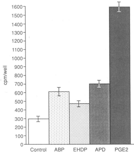
Figure 8. Adenylate cyclase activity in chicken osteoclasts. Chicken osteoclasts were incubated with 1 \mu Ci [ 3 H]adenine for 2 h at 37°C, washed, and then incubated with 1 mM isobutyl methylxanthine in the absence or presence of 0.1 mM ABP, EHDP, APD, or 1 \mu M prostaglandin E 2 for 10 min. [ 3 H] cAMP was column separated from other nucleotides and counted as described previously by Salomon et al. (53). For three sets of experiments ( n = 3-4 each), no significant cyclase response was observed for ABP, EHDP, or APD compared to PGE 2 (mean \pm SD). □, basal; ▤, ABP; ▥, EHDP; ▧, APD; ▨, PGE 2 .
