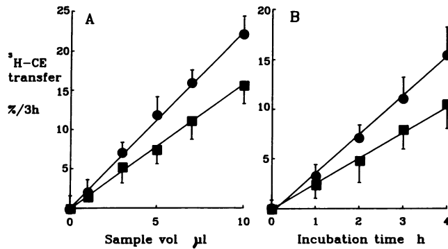
Figure 2. Relationship of CETP activity assay to CETP concentration (A) and incubation time (B). (A) Volumes of up to 10 \mu\text{l} of normolipidemic plasma (●) or purified CETP (■, 200 \mu\text{g} protein/ml) were incubated for 3 h at 37°C with ^3\text{H} -CE-HDL 3 (25 nmol CE) and unlabeled LDL (500 nmol CE) in 50 mM Tris, 150 mM NaCl, 2 mM EDTA, pH 7.4 in a final vol of 100 \mu\text{l} . (B) 5 \mu\text{l} of normolipidemic plasma (●) or purified CETP (■) were incubated under the same conditions as in A for the indicated times. After the incubations, LDL were precipitated using heparin and \text{MnCl}_2 . CETP activity was determined from the loss of ^3\text{H} -CE from the HDL supernatant, minus the loss from blank samples incubated for the same time without plasma or purified CETP. Points are expressed as mean \pm SD of quadruplicate determinations.
