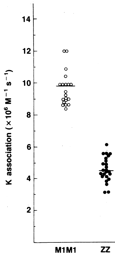
Figure 4. Association rate constants ( K association) of M1-type and Z-type \alpha 1 AT for human neutrophil elastase. Neutrophil elastase and the M1 or Z-type \alpha 1 AT were incubated for various times as shown in Fig. 3, the half time of the reaction was determined, and the K association calculated. Each data point represents the K association calculated from individual samples of PiM1M1 and PiZZ individuals; there were 20 samples from 7 PiM1M1 individuals and 24 samples from 10 PiZZ individuals. For each sample, each time point was determined in triplicate. The horizontal line represents the mean for each group.
