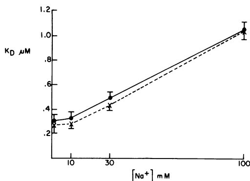
Figure 4. Affinity of intact platelet \alpha_2 -adrenoreceptors for L-epinephrine in isotonic assay media containing varying sodium concentrations. Mean \pm SEM for five normotensive (solid line) and five hypertensive (dashed line) subjects.
