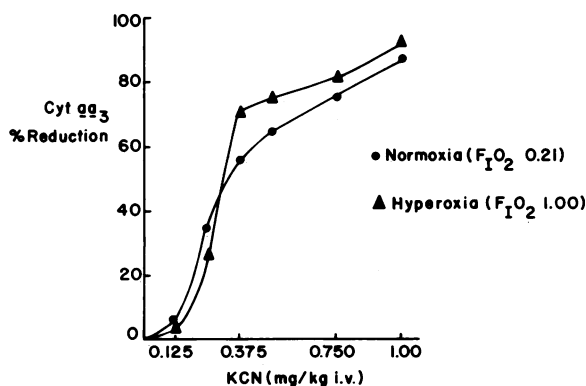
FIGURE 4 Cyanide-cytochrome dose-response curves: KCN vs. percentage reduction of cytochrome ( t_{1/2} off). Dose of KCN (milligram per kilogram, intravenous) was plotted against P_{max} (Fig. 2) expressed as a percentage of the total labile signal (Fig. 3). Hyperoxia had no effect on the position of the dose-response curves.
