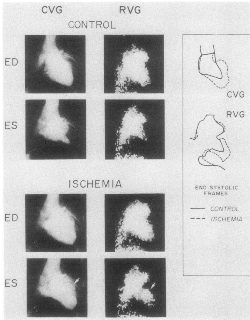
FIGURE 4 A large region of ischemia. There was 35.07 g of ischemic tissue, which caused 45.6% ACS on CVG and 44.4% on RVG.
