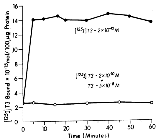
FIGURE 6 Time-course of binding of [ 125 I]T3 to GH 1 cell nuclear extract at 37°C. GH 1 cell nuclear extracts (60 μg protein) and buffer controls were incubated with [ 125 I]T3 ( 2 \times 10^{-10} M) as well as with [ 125 I]T3 plus a 250-fold molar excess of nonradioactive T3. The samples were incubated at 37°C, and at the indicated times, the bound [ 125 I]T3 was determined as described in Methods. Each point reflects subtraction of the [ 125 I]hormone determined with the buffer control ( 1.5 \times 10^{-15} mol [ 125 I]T3). Each point reflects the mean of three determinations, and each determination did not vary more than 12% from the mean.
