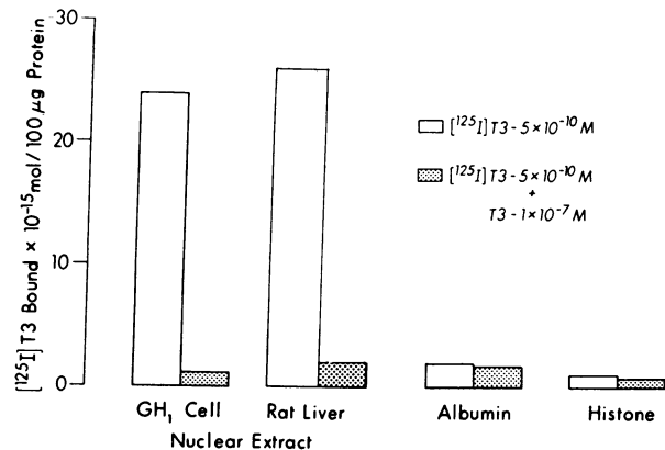
FIGURE 2 Binding of [ ^{125} I]T 3 with GH 1 cell and rat liver nuclear extract, albumin, and histone. GH 1 cell nuclear extract (55 \mu g protein), rat liver nuclear extract (75 \mu g protein), crystalline bovine serum albumin (75 \mu g protein), histone (75 \mu g protein), and a buffer control were incubated with the concentrations of T 3 indicated in the figure. After a 2-h incubation at 0°C, the bound and free hormone were separated as described in Methods. Each point reflects subtraction of the [ ^{125} I]T 3 determined with the buffer control ( 0.83 \times 10^{-15} mol [ ^{125} I]T 3 ). Each point represents the mean of three determinations. Each determination did not vary more than 10% from the mean.
