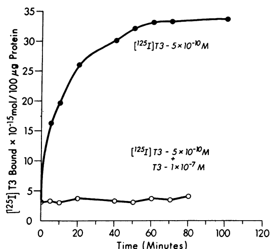
FIGURE 5 Time-course of binding of [ 125 I]T3 to GH 1 cell nuclear extract at 0°C. GH 1 cell nuclear extracts (70 μg protein) and buffer controls were incubated with [ 125 I]T3 ( 5 \times 10^{-10} M) as well as with [ 125 I]T3 plus a 200-fold molar excess of nonradioactive T3. The samples were incubated at 0°C, and at the indicated times, the bound [ 125 I]T3 was determined as described in Methods. Each point reflects subtraction of the [ 125 I]hormone radioactivity determined with the buffer control ( 1.1 \times 10^{-15} mol [ 125 I]T3). Each point reflects the mean of three determinations, and each determination did not vary more than 10% from the mean.
