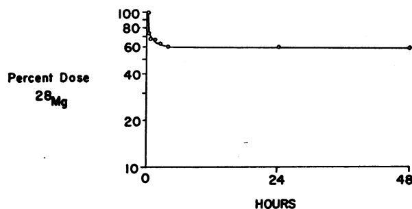
FIGURE 2 Example of ^{28}\text{Mg} exchange with bone magnesium. The disappearance of ^{28}\text{Mg} from the incubating media is shown over the first 48 h.
