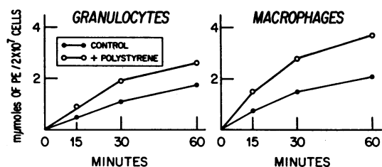
FIGURE 7 Synthesis of phosphatidylethanolamine (PE) from medium lysophosphatidylethanolamine (LPE) with and without particles. Results are means of two closely similar experiments carried out with granulocytes at LPE concentrations of 0.07 and 0.12 mmole/liter and of three macrophage experiments at LPE concentrations of 0.04, 0.06, and 0.1 mmole/liter.
