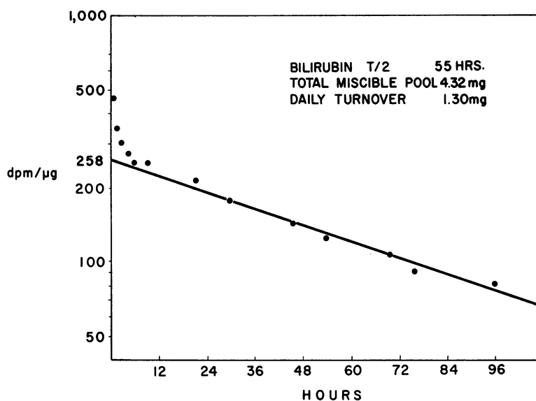
FIG. 2. SA OF SERUM BILIRUBIN IN A 400-G MALE GUNN RAT WITH EXTERNAL BILIARY DRAINAGE. At time zero, 0.64 \mu c C^{14} -bilirubin was injected intravenously.
