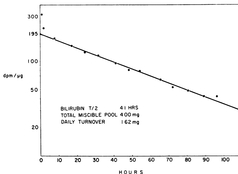
FIG. 3. SA OF SERUM BILIRUBIN IN A 355-G MALE GUNN RAT WITHOUT EXTERNAL BILIARY DRAINAGE. At time zero, 0.46 \mu\text{C} C 14 -bilirubin was injected intravenously.
