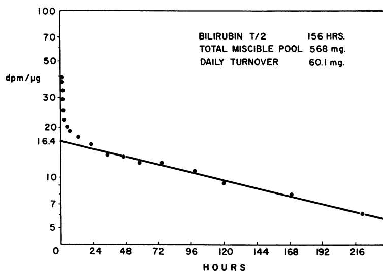
FIG. 1. SA OF SERUM BILIRUBIN IN THE 4½-YEAR-OLD PATIENT WITH CONGENITAL UNCONJUGATED HYPERBILIRUBINEMIA. At time zero, 4.3 \mu\text{C}^{14} -bilirubin was injected intravenously.
